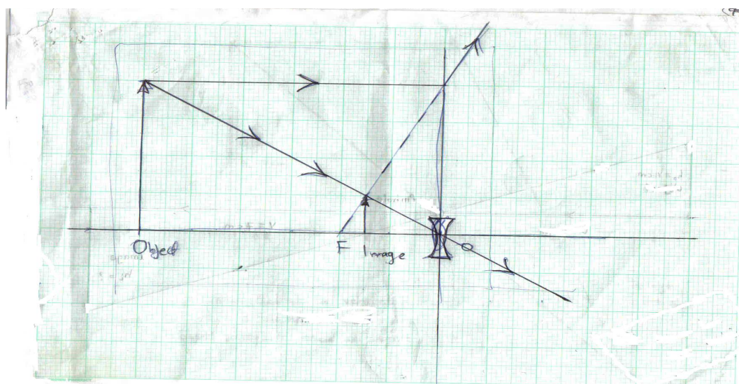
Figure 2.4: Ray diagram: Diverging lens
