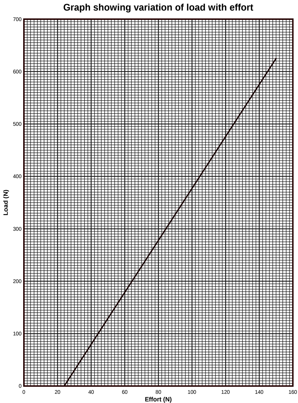
Figure 1.1: Graph of Load against Effort
