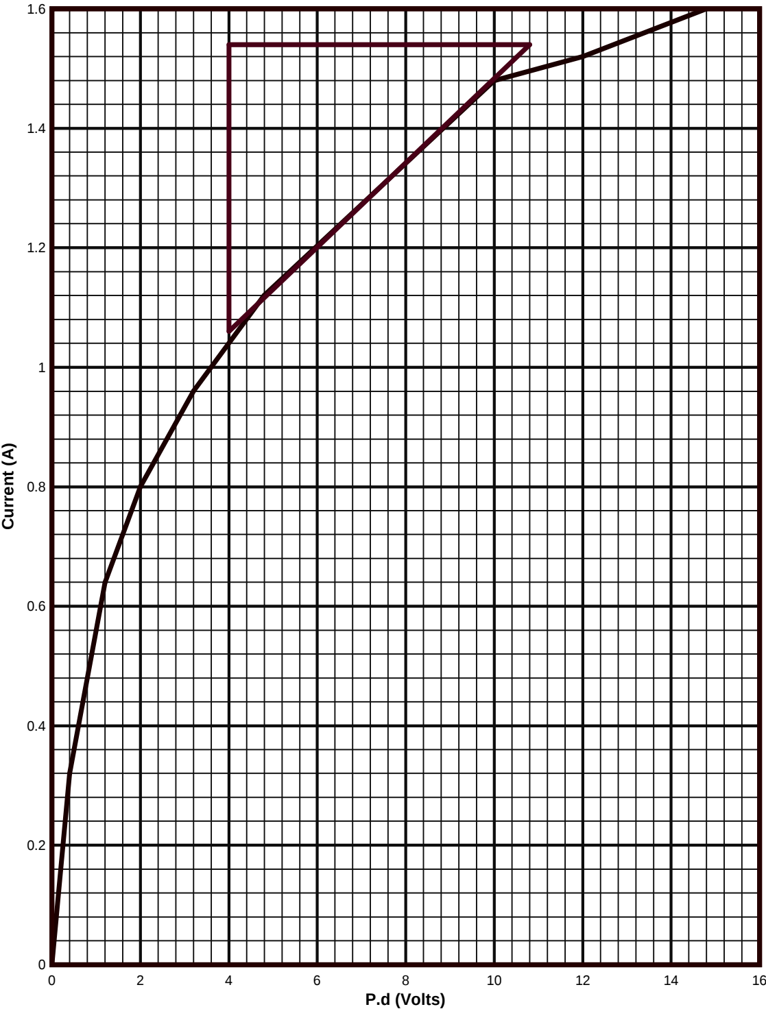
Figure 4.2: Graph of Current against Voltage
