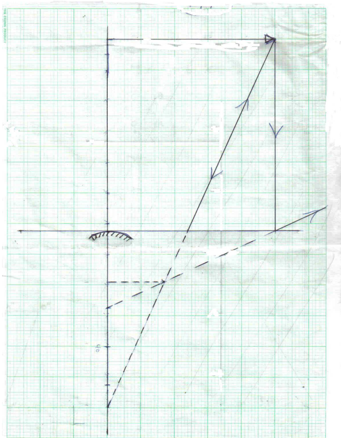
Figure 2.2: Scaled ray diagram: curved mirrors
