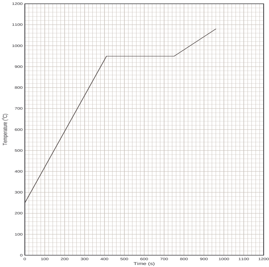
Figure 3.1: Graph of Temperature against time
