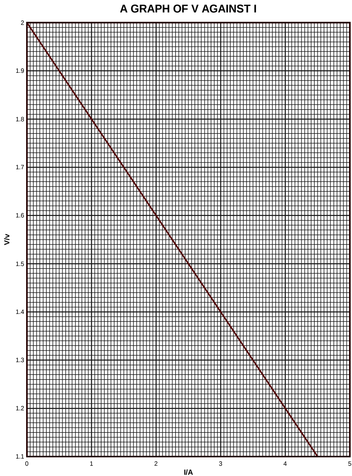
Figure 4.1: Graph of Voltage versus current
